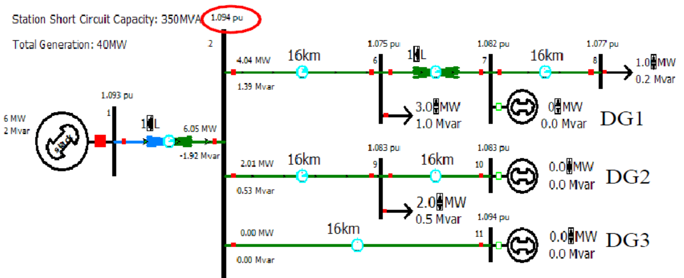
Fig. 66 MV Network used in a DER interconnection case study [31]
