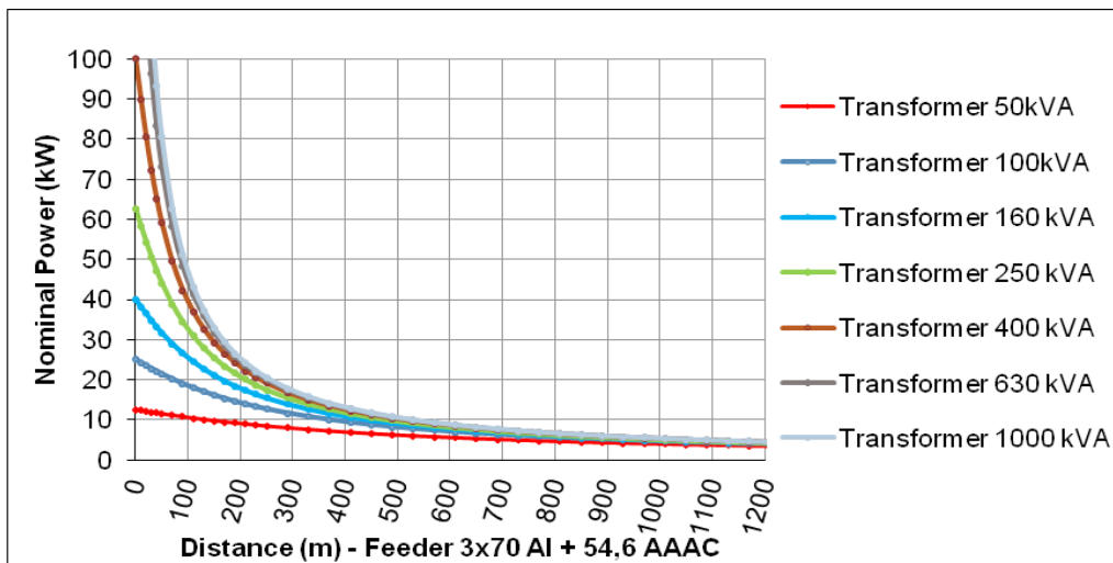
Fig. 15 Maximum permitted small WT capacity, as a function of the connection point distance from the feeder origin, for different MV/LV transformer capacities (Greece).
