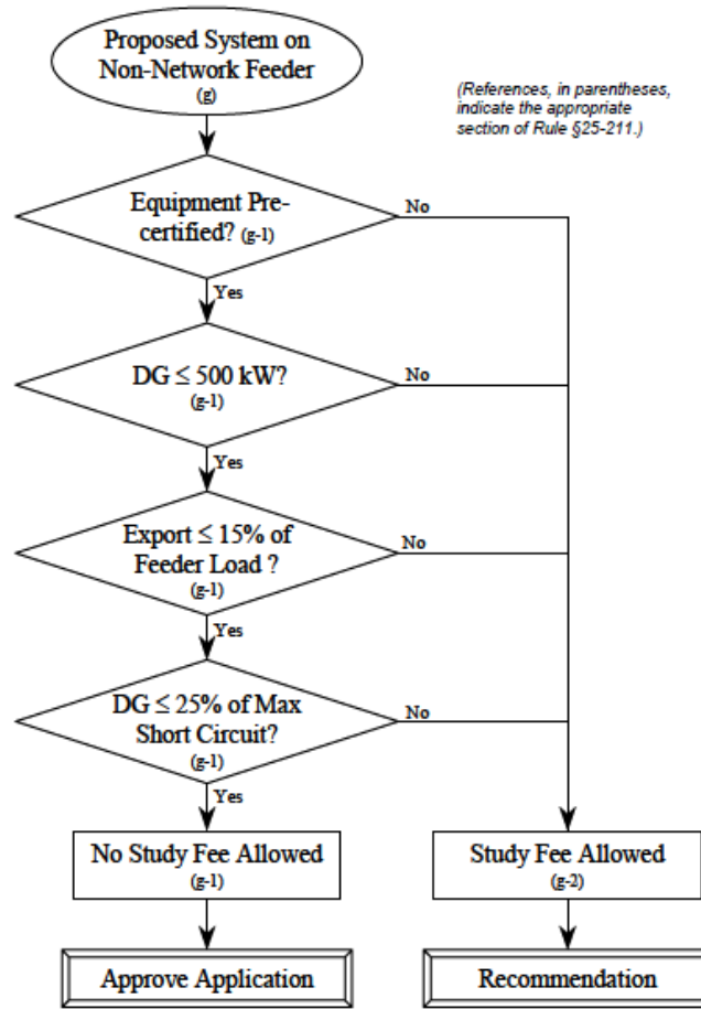
Fig. 34 Flow chart of interconnection process (USA - Texas) [84]
