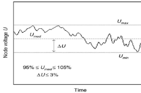
Fig. 13 Voltage variation due to DER interconnection at a node and steady state voltage variation limits (Greece)
