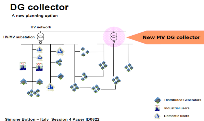
Fig. 52 New network planning for high DER penetration (Italy) [61]
