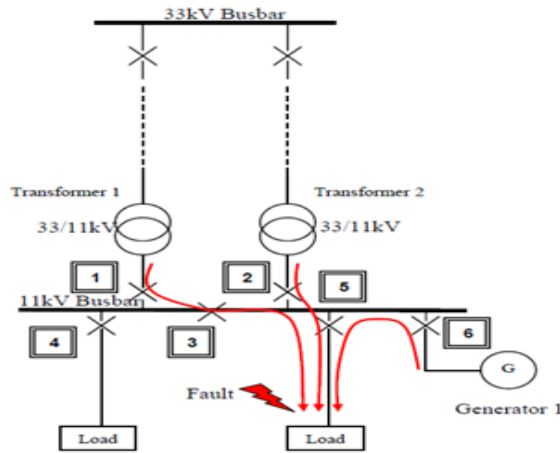
Fig. 58 Addressing the short-circuit issue by implementing sequential switching [103]
