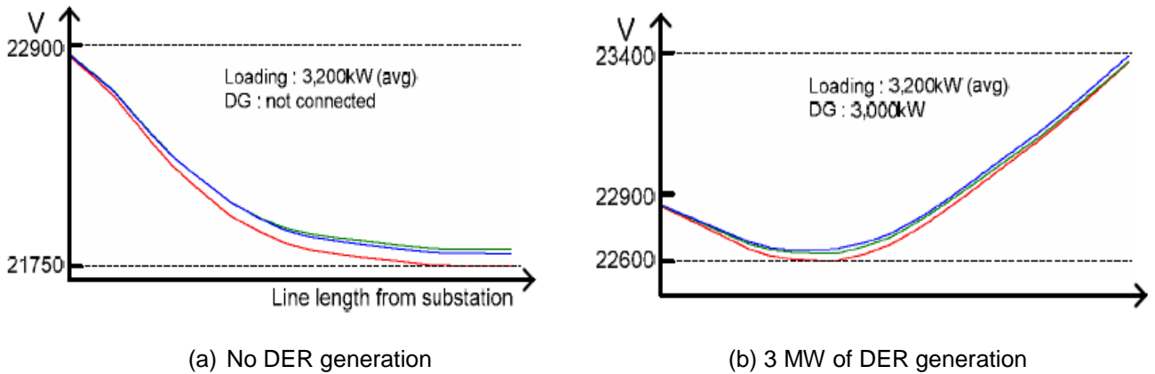
Fig. 82 Average load 3000kW and DG interconnection voltage profile
