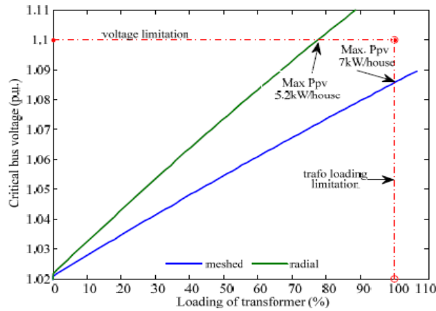
Fig. 68 Solar PV integration levels without Q control and grid constraints [104]
