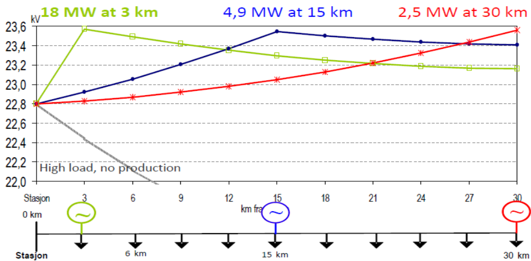
Fig. 20 Feasible generation levels at different locations
