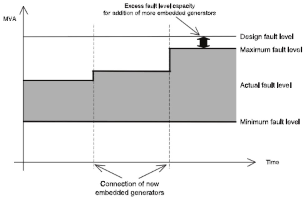
Fig. 1 Impact of DER on actual fault level and DER hosting capacity based on design fault level [1]
