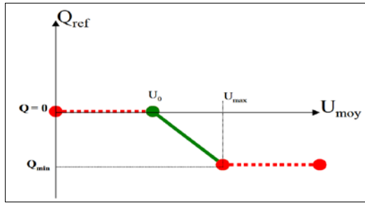
Fig. 48 Reactive power control in case of overvoltage situation
