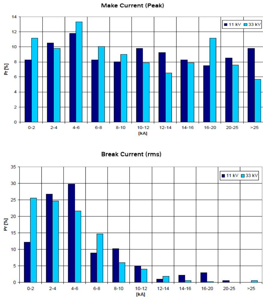
Fig. 29 Distribution of Headroom Availability in Urban MV Networks (UK) [9]
