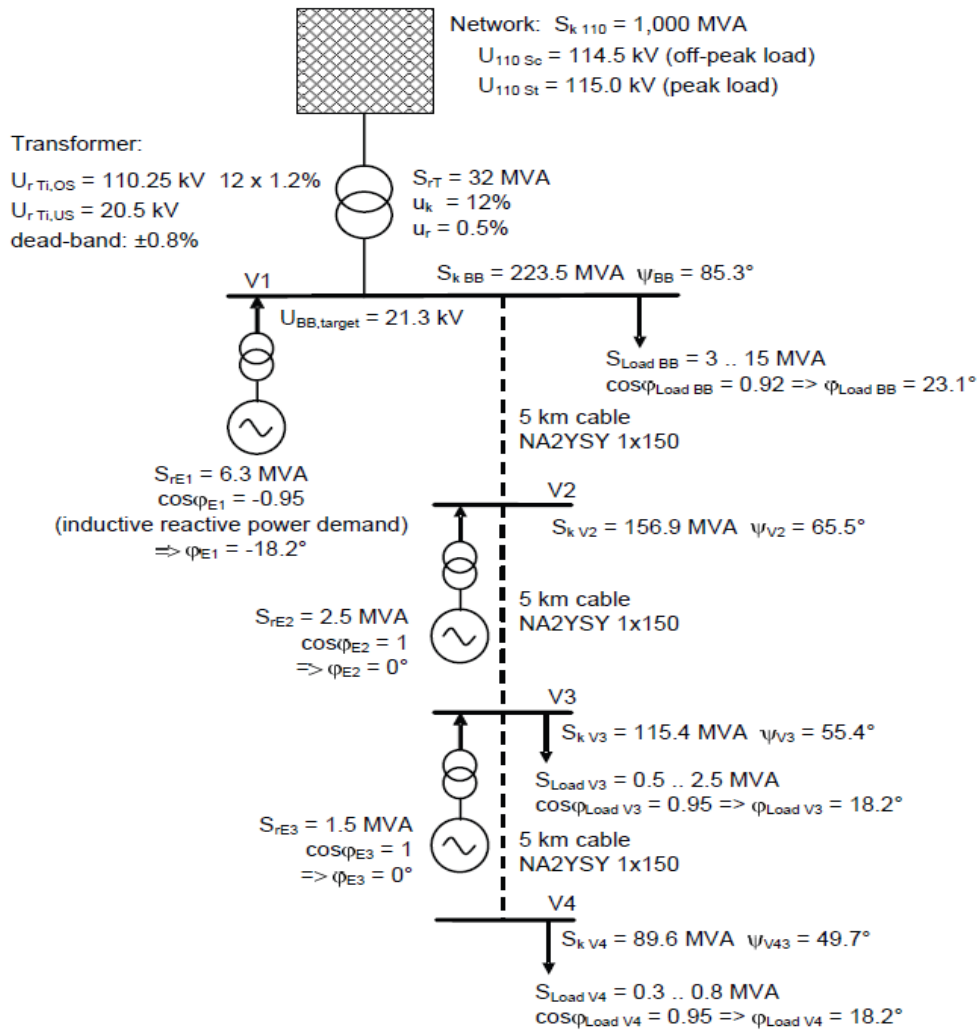
Fig. 62 MV network used in a DER interconnection case study [17]
