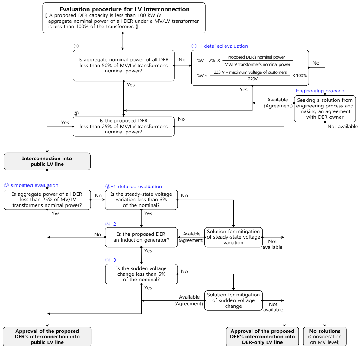
Fig. 28 Flow chart that shows the technical methodology implemented in LV networks (South Korea)
