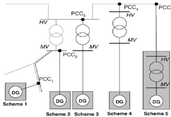
Fig. 12 Typical DER interconnection schemes at MV level (Greece)
