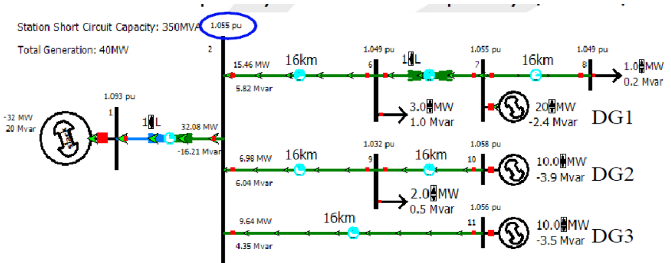
Fig. 65 MV Network used in a DER interconnection case study [31]
