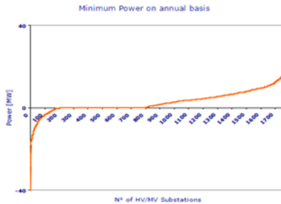
Fig. 18 Minimum active power (MW) on annual basis of HV/MV substations in Enel network (Italy) [61]
