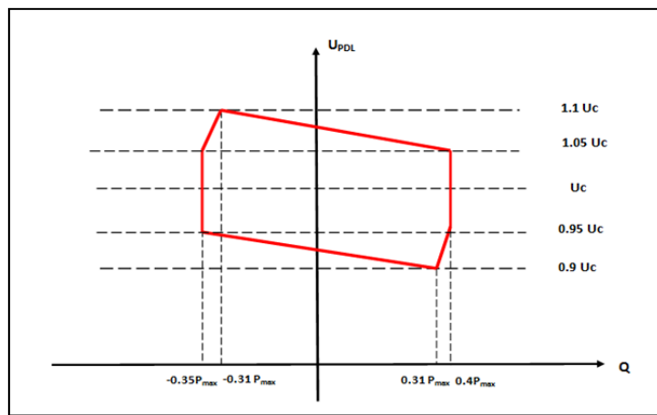
Fig. 51 Power factor control
