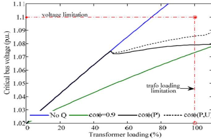
Fig. 69 Estimation of PV penetration in the radial distribution grid with different Q control methods [104]
