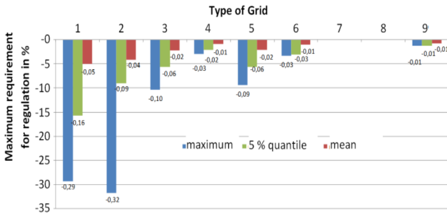
Fig. 77 Required regulation capabilities
