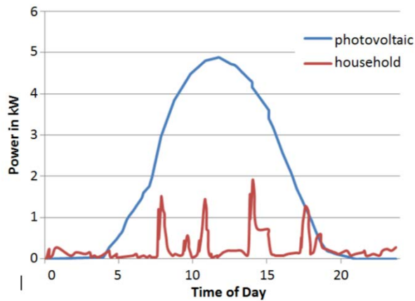
Fig. 70 PV Feed –in and household load in summer
