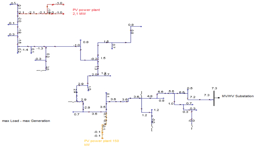
Fig. 79 MV network used for a DER interconnection case study
