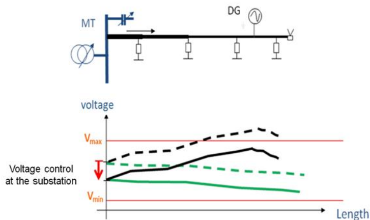
Fig. 46 On Load Tap Changer in coordinated voltage control
