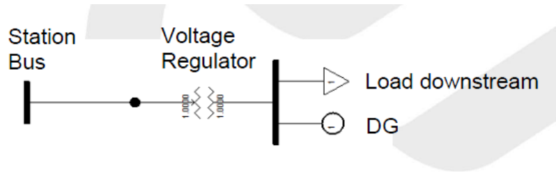
Fig. 3 Network in which unacceptable post-contingency voltage may occur [29]
