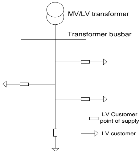
Fig. 22 Shared LV feeder (loads and DER)
