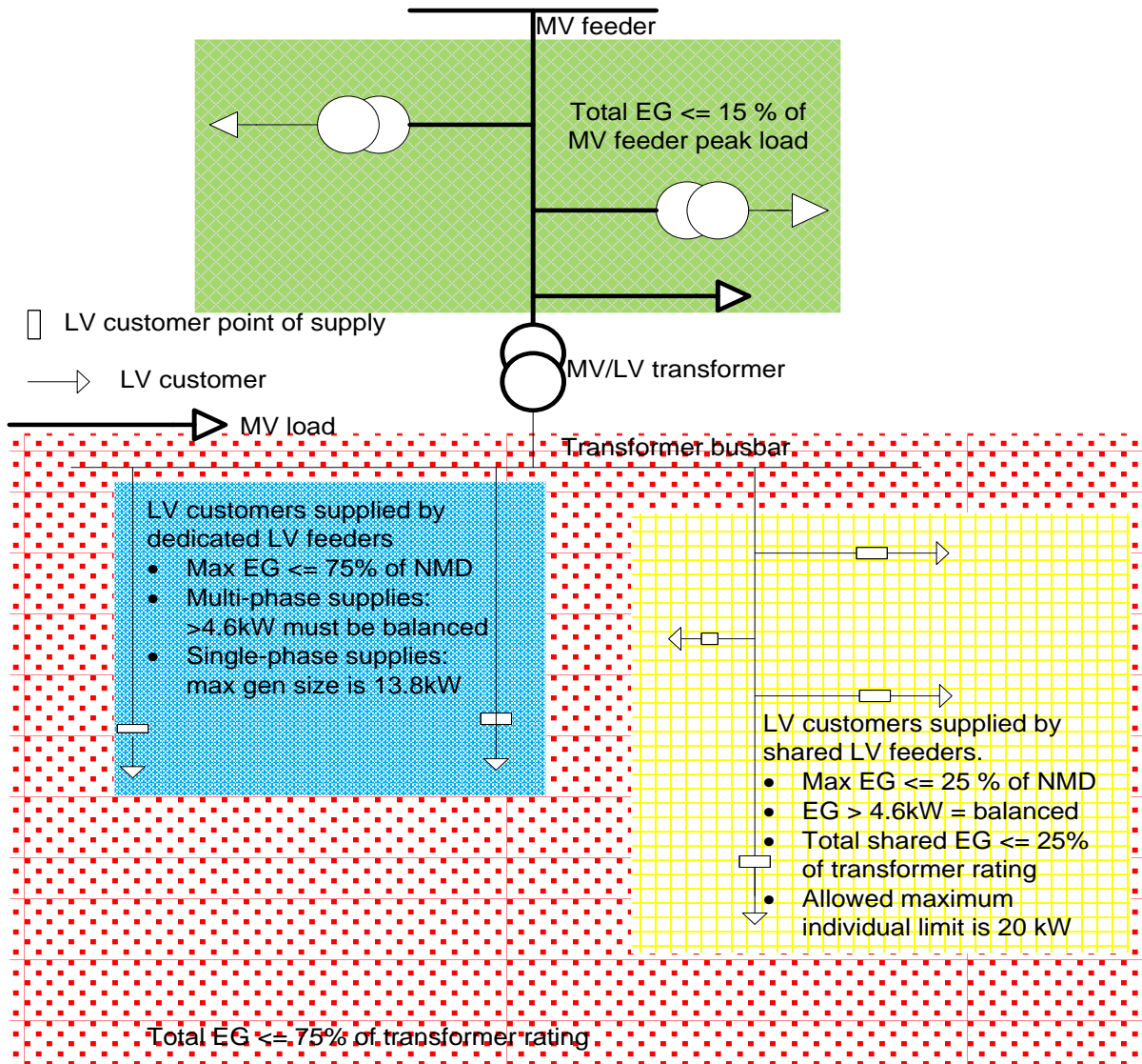
Fig. 25 Summary of simplified connection criteria (South Africa)
