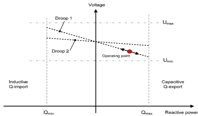
Fig. 45 Q-V DER control (droop function) [45]
