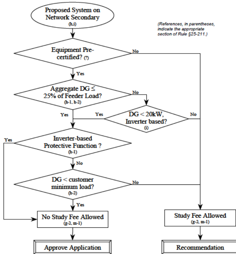
Fig. 35 Flow chart of interconnection process in LV networks (USA - Texas) [84]
