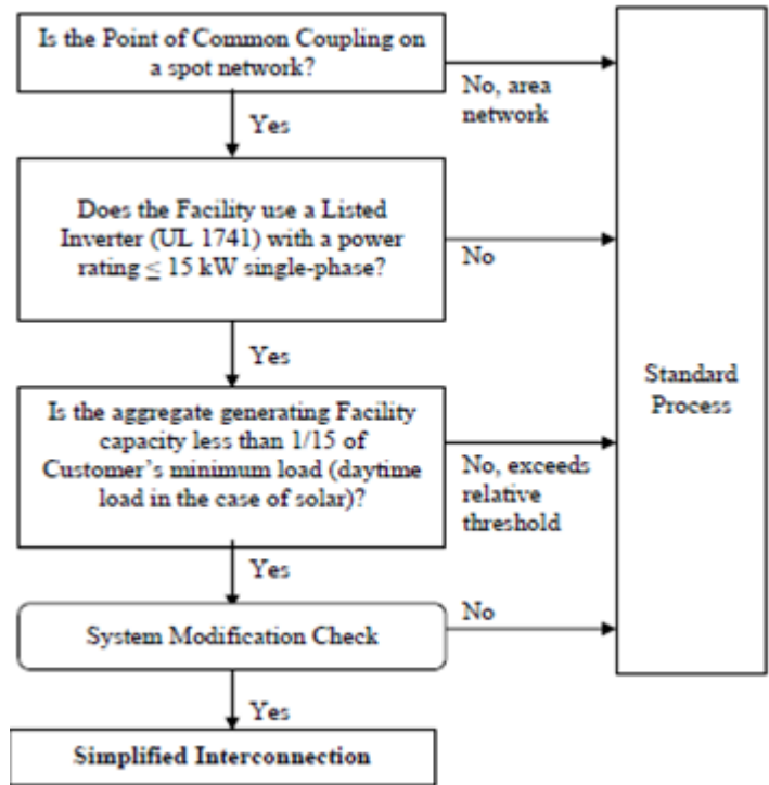
Fig. 33 Simplified Interconnection to Networks (USA - Massachusetts) [83]
