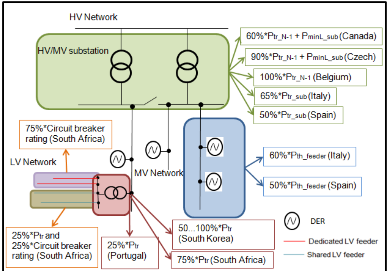
Fig. 60 Criteria related to or based on ratings/thermal limits
