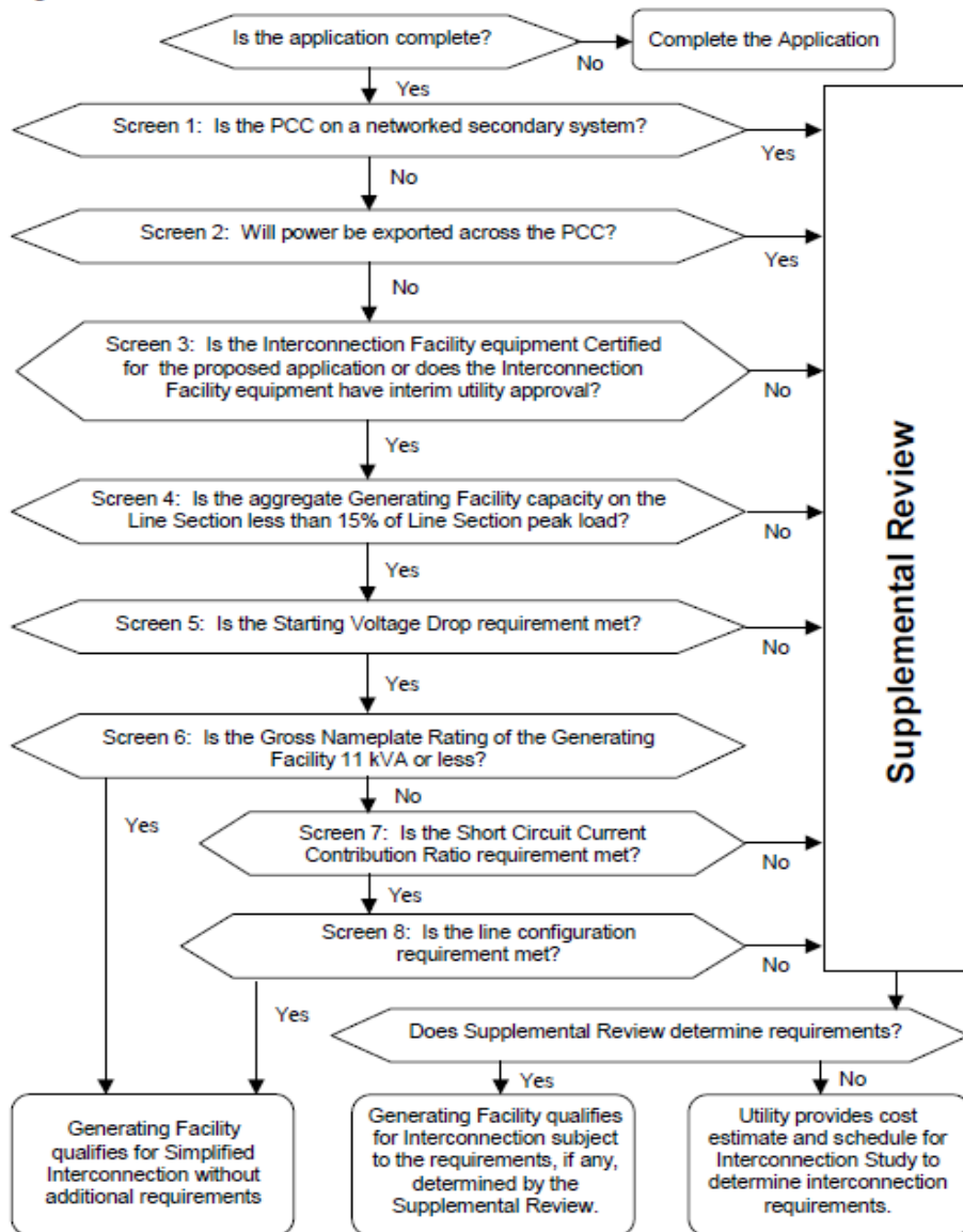
Fig. 30 Flow chart of screening criteria (USA - California) [80]
