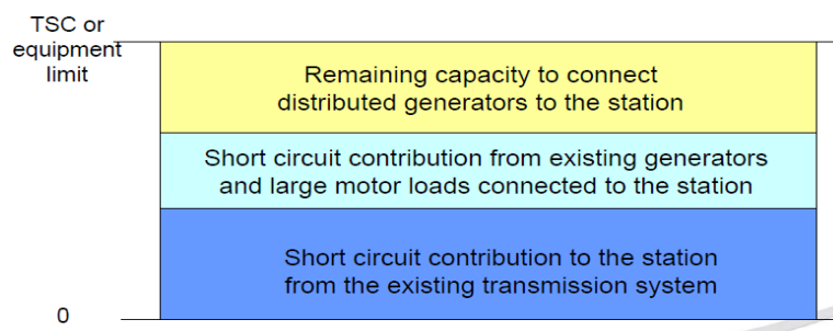
Fig. 8 Impact of DER on short-circuit levels (short-circuit capacity) [35]
