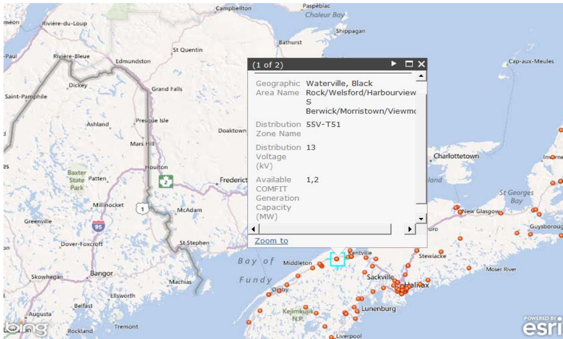
Fig. 39 Map showing available DER capacity (Canada - Nova Scotia) [93]
