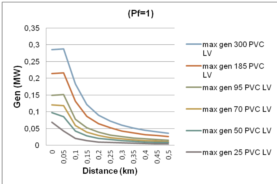
Fig. 24 Dedicated LV feeder maximum gen sizes as a function of cable size and distance (South Africa)
