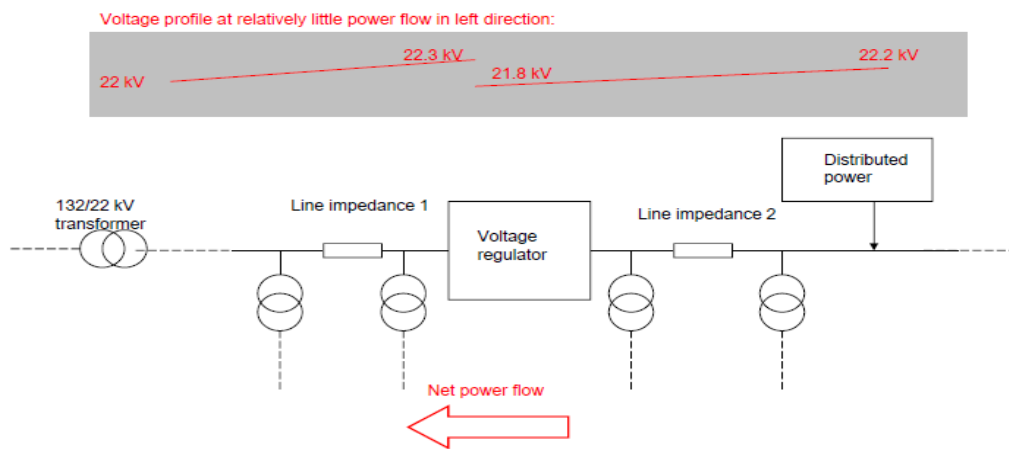
Fig. 54 A presentation of the voltage booster. MV voltage booster prototype is currently being tested
