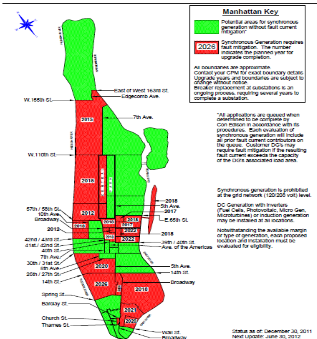
Fig. 42 Map showing the available short-circuit DER capacity (USA – New York)
