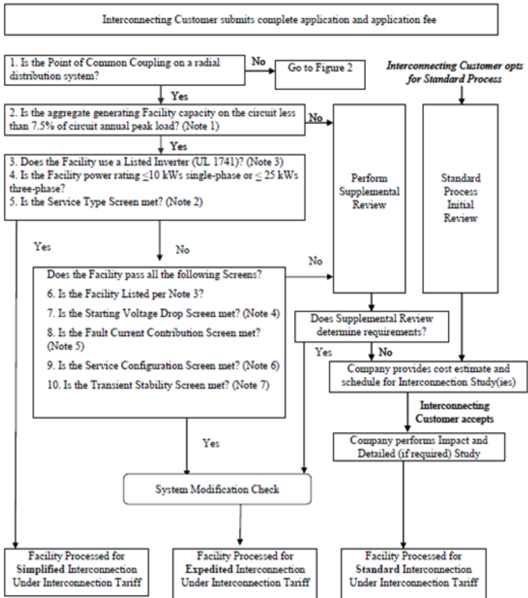
Fig. 32 Schematic of Massachusetts DG Interconnection Process (USA - Massachusetts) [83]
