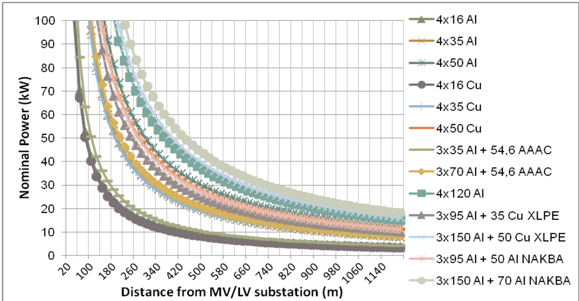
Fig. 14 Maximum permitted DER capacity for different types of LV feeders, as a function of the connection point distance from the feeder origin (Greece).
