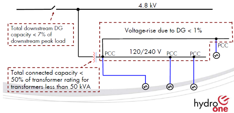
Fig. 7 DER hosting capacity rules in LV networks (Canada - Hydro One Inc.) [33]
