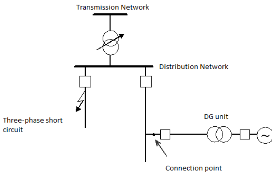
Fig. 21 Dimensioning fault – Fault ride through capabilities
