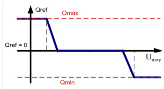
Fig. 50 Reactive power control using a voltage dead band
