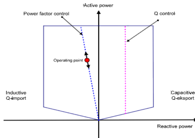
Fig. 44 Power factor and reactive power control of DER [45]
