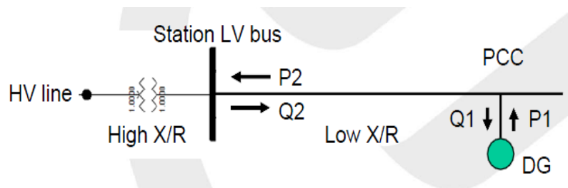
Fig. 4 Network in which high aggravation of voltage fluctuation may occur [29]
