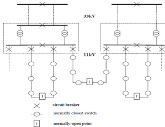
Fig. 56 Addressing the short-circuit issue by making network reconfiguration [103]
