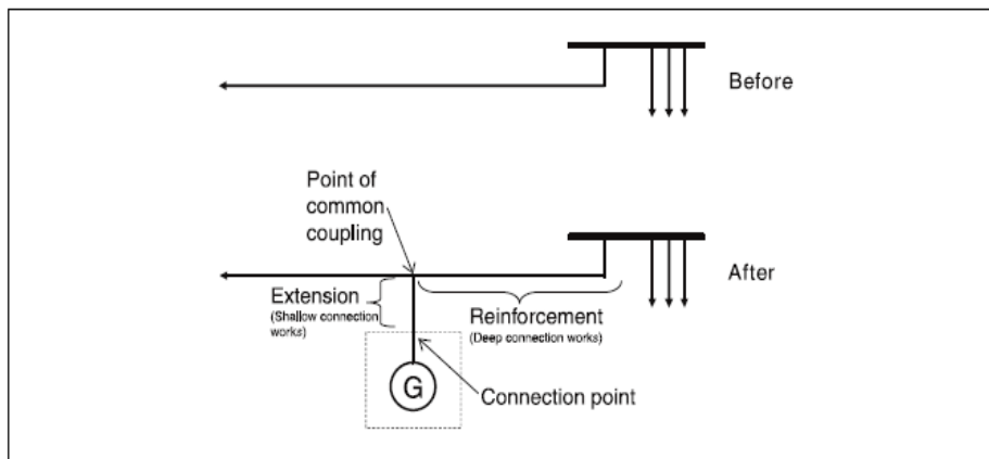
Fig. 43 Possible interconnection works [1]
