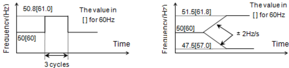
(a) For step change in frequency (b) For ramp change in frequency Fig. 36 FRT requirements for PV systems in Japan
