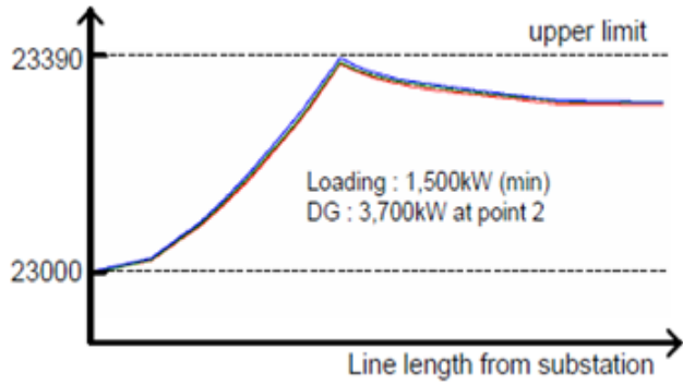
Fig. 84 The voltage profile for 3700kW DG interconnection at point 2(15km location from substation) in the condition of minimum voltage margin
