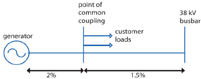
Fig. 17 Upper permitted voltage rise (Ireland) [2]
