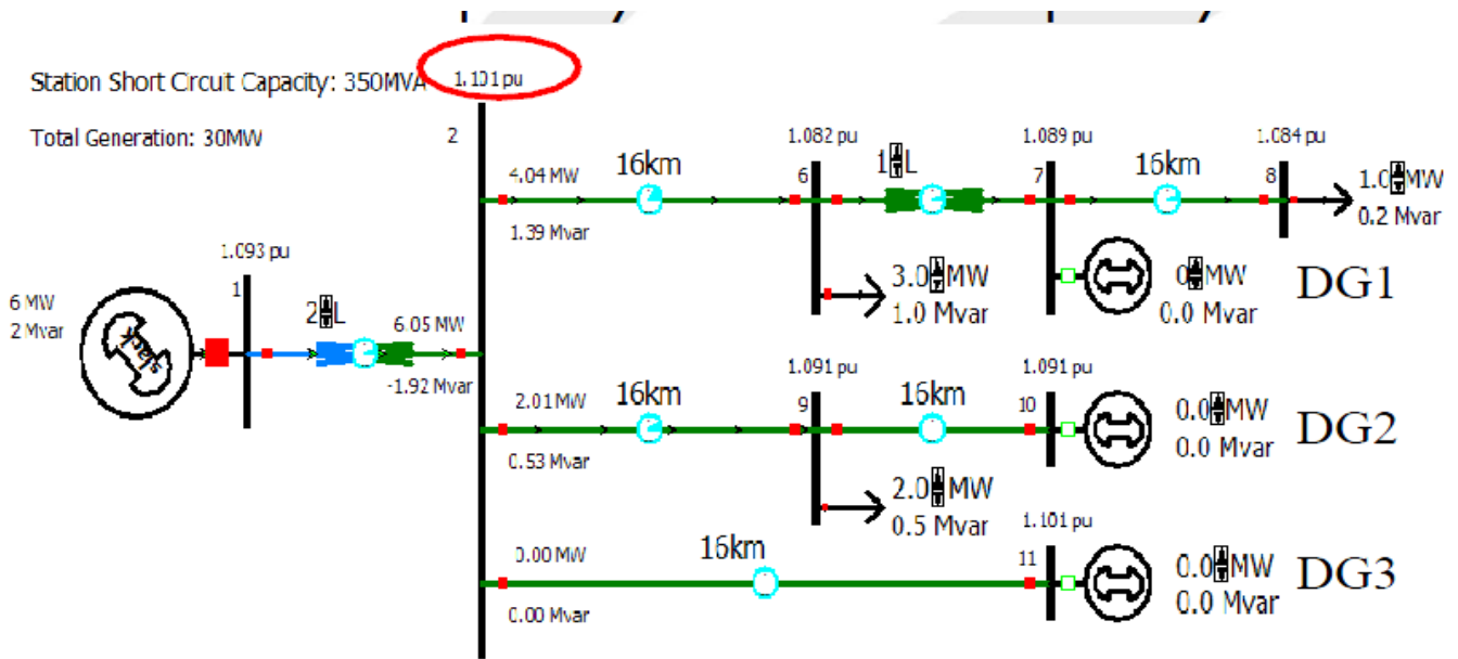
Fig. 64 MV Network used in a DER interconnection case study [31]
