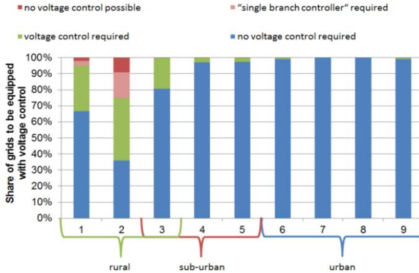
Fig. 76 Types of voltage control in different LV grids
