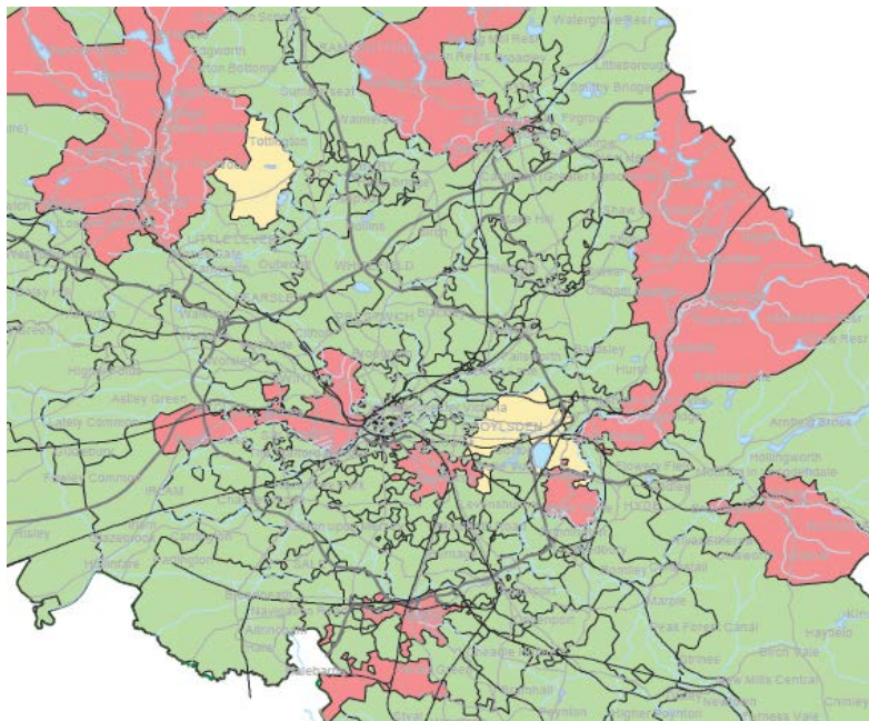
Fig. 40 Map showing the available substation short-circuit DER capacity (UK – Electric Northwest) [96]
