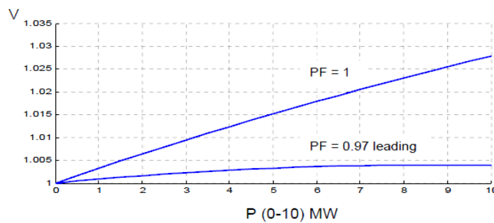
Fig. 6 Voltage variation of PCC depending on power factor of DG [30]
