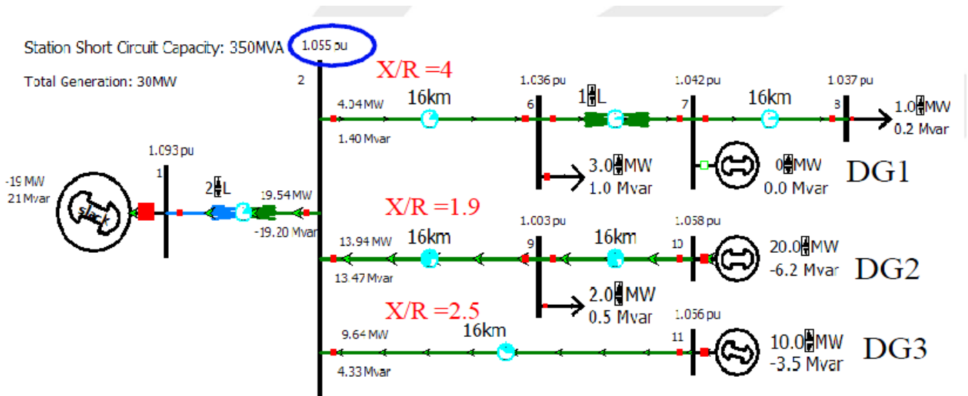
Fig. 63 MV Network used in a DER interconnection case study [31]
