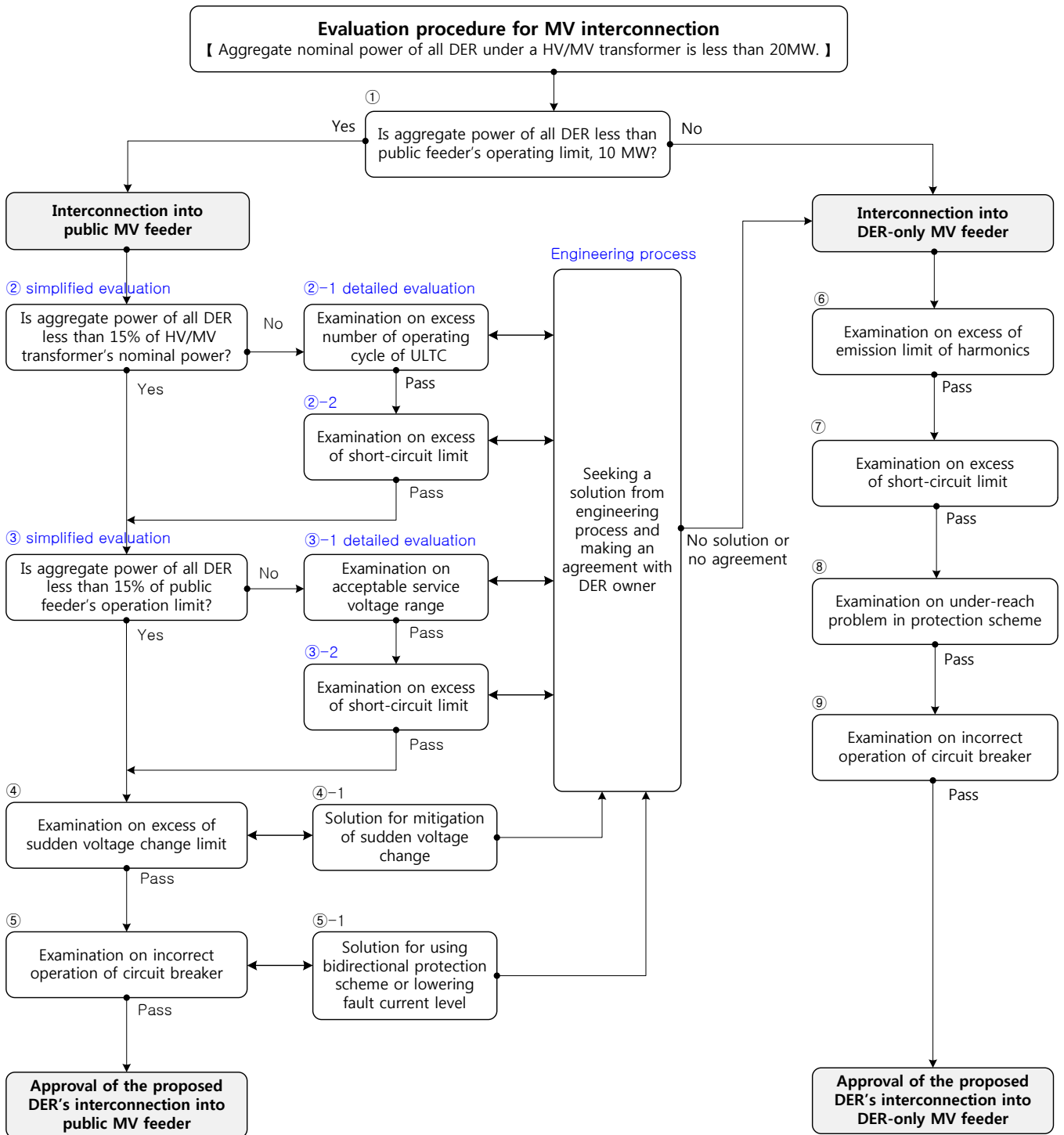
Fig. 27 Flow chart that shows the technical methodology implemented in MV networks (South Korea)
