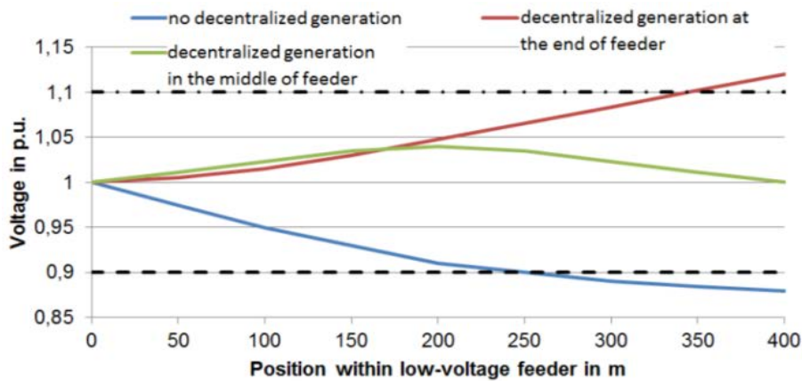
Fig. 73 Exemplary voltage profiles
