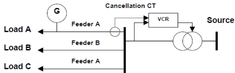
Fig. 59 Cancellation CT and Line Drop Compensation (LDC) [103]
