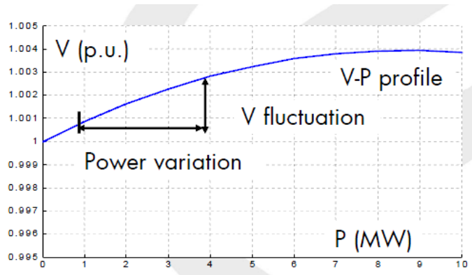
Fig. 5 Short-term voltage fluctuation according to Hydro One Inc. definition [31]
