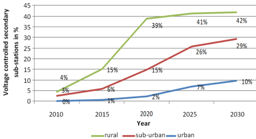
Fig. 75 Voltage-controlled substations requires in rural, urban and sub-urban grids
