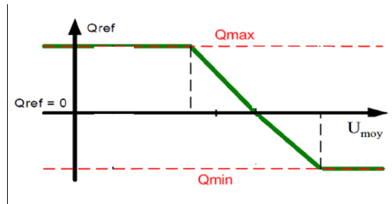
Fig. 49 Reactive power control (general concept)
