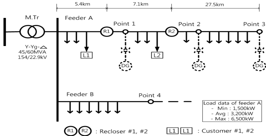
Fig. 81 Targeted distribution system
