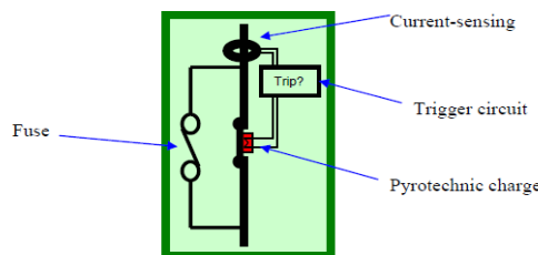
Fig. 57 Addressing the short-circuit issue by using Is limiter [103]
