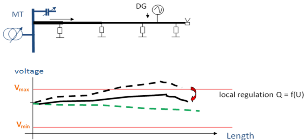
Fig. 47 DER (local) reactive compensation for voltage regulation
