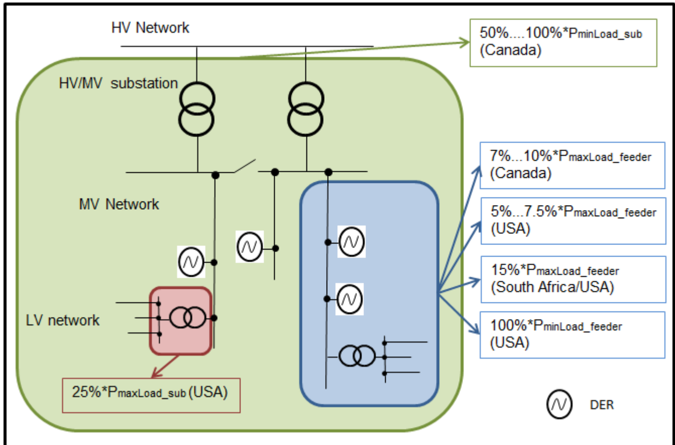
Fig. 61 Criteria based on the load-to-generation ratio
