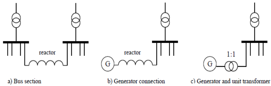
Fig. 55 Addressing the short-circuit issue by increasing PCC impedance [103]
