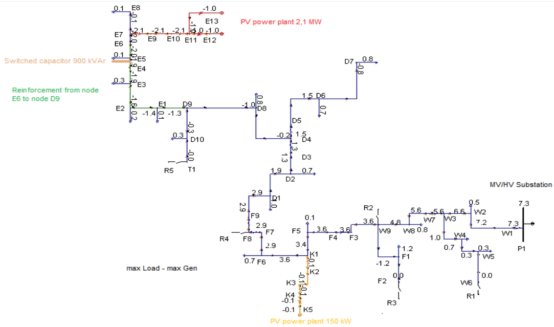
Fig. 80 MV network used for a DER interconnection case study
