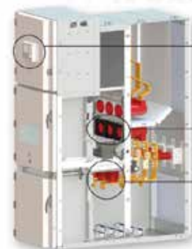
1. Redundant protection relay with IEC 61850 2. Current sensor 3. Voltage sensor
