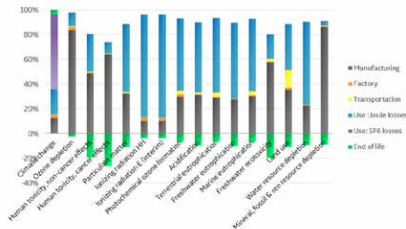
Figure 3: Life Cycle Assessment results for the F35-145kV (SF 6 )
